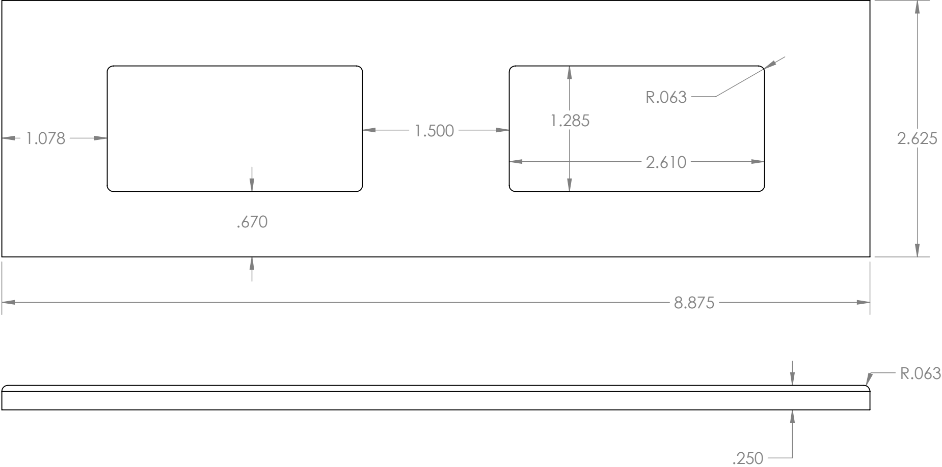
Top Plate, Brass, hammered texture, Full Scale
