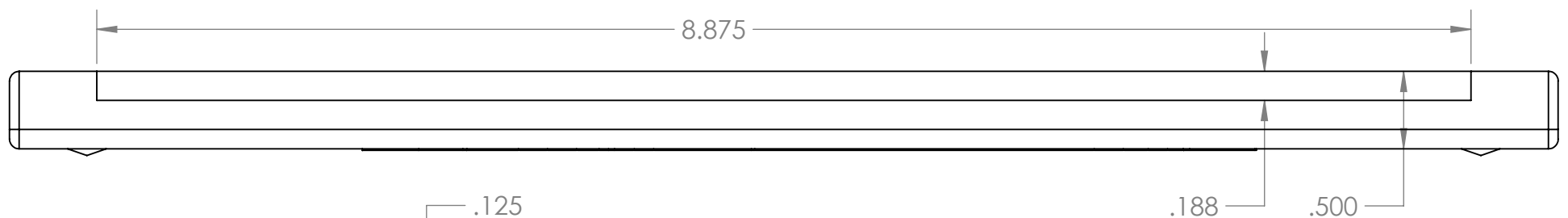
End, Sapele, Ebony Plugs, Full Scale
